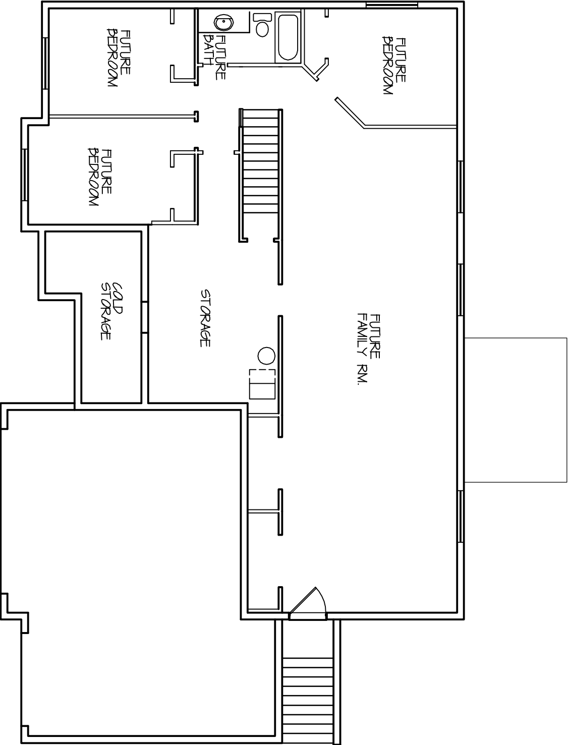
BASEMENT PLAN 1912 RAMBLER PLAN 1874 SQ. FT.
